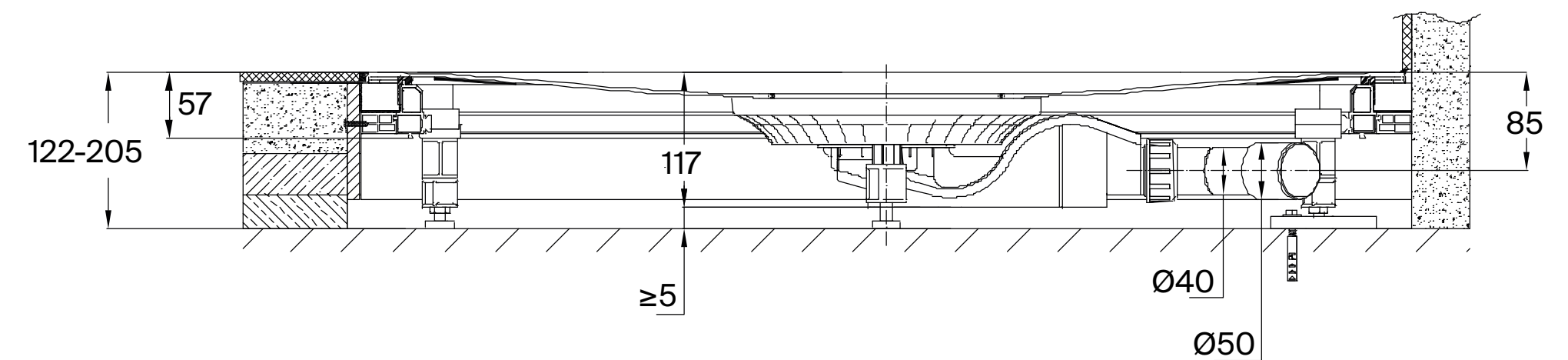
Representation Universal installation system with waste fitting BetteAir 50 – 0.6 l/s, with water drainage on the side, standard-compliant water seal depth 50 mm to EN 274
