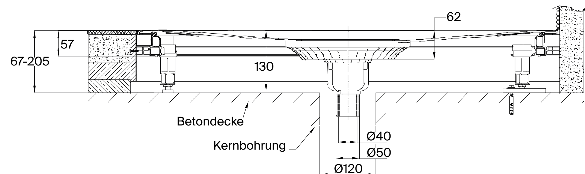
Representation Universal installation system with waste fitting BetteAir Down 0.6 l/s, with vertical water drainage, water seal depth 50 mm
